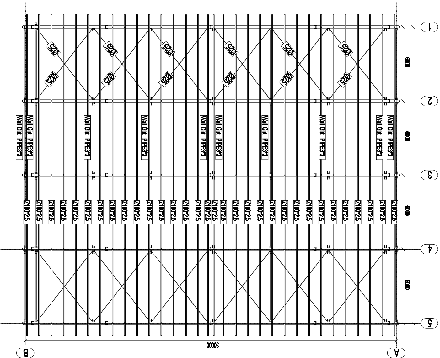
PLAN +7200
