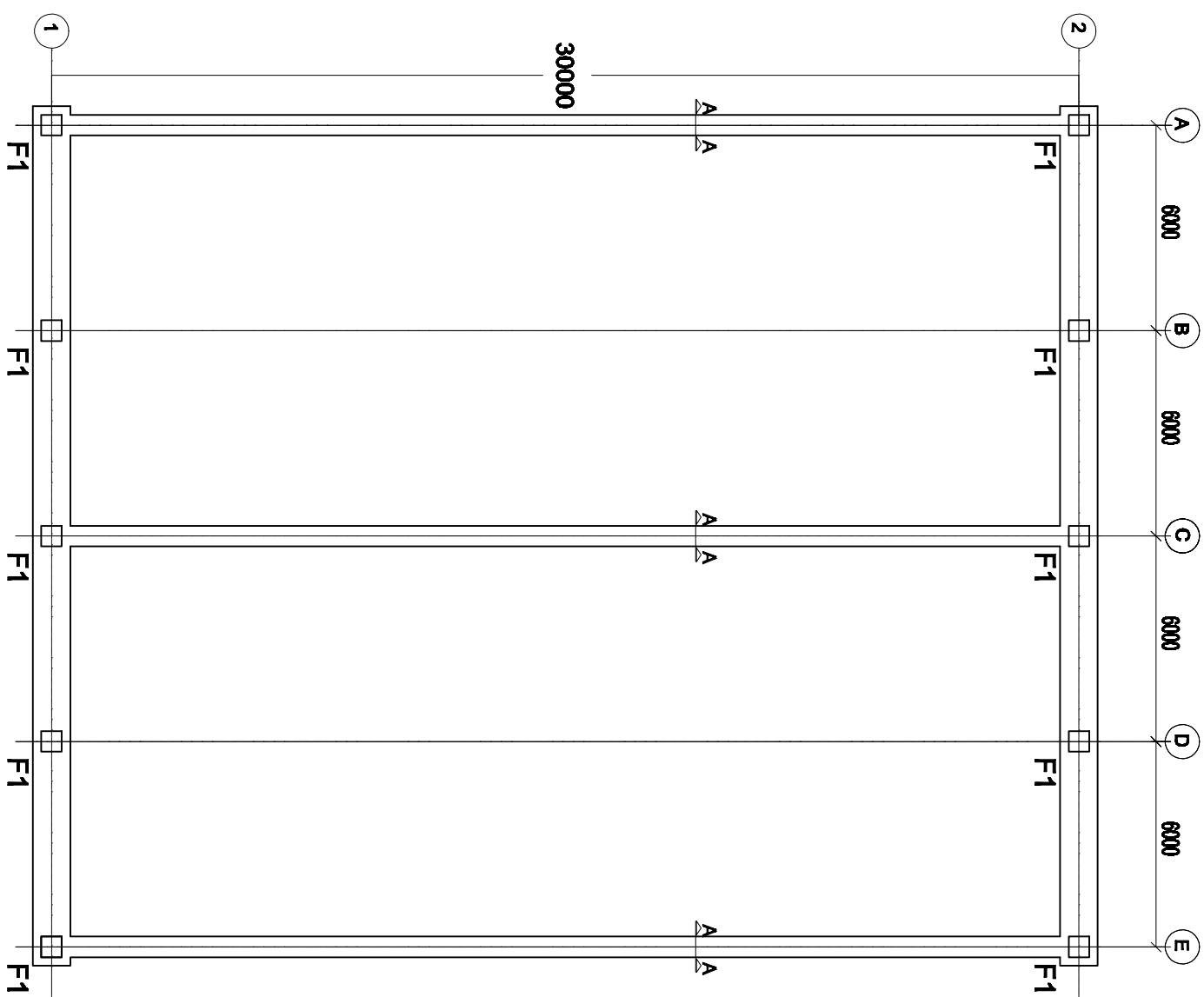
FOUNDATION PLAN Scale 1/200
